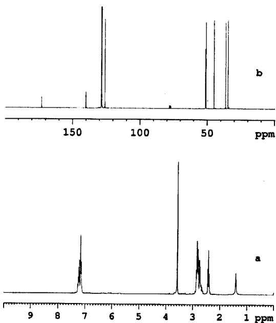
^1\text{H} (a) and \{^1\text{H}\}^{13}\text{C} (b) NMR spectra (in \text{CDCl}_3 ) of 3 Fig. 1
