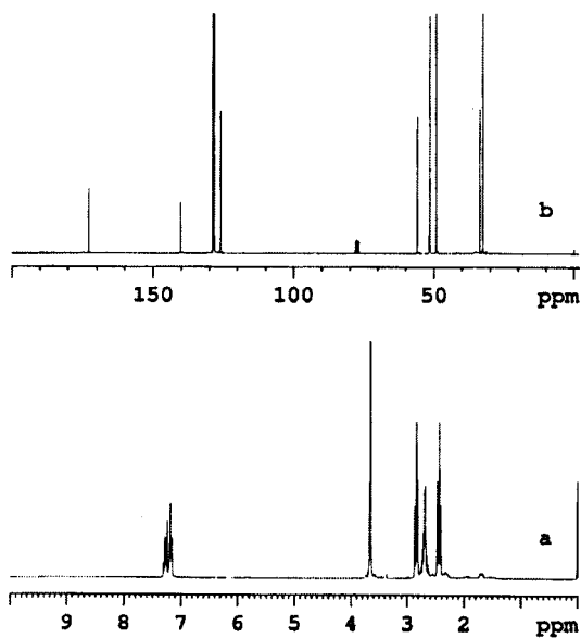
^1\text{H} (a) and \{^1\text{H}\}^{13}\text{C} (b) NMR spectra (in \text{CDCl}_3 ) of 4 Fig. 2
